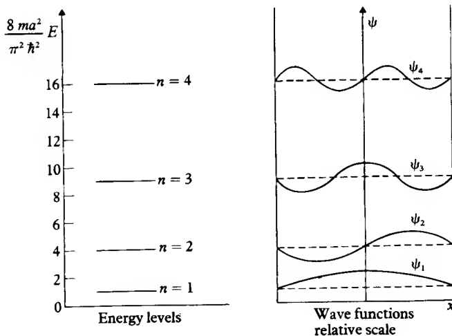
2.2 (a) The infinite square well
